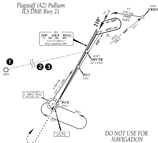
Figure 6-73 ILS Approach, Flagstaff
